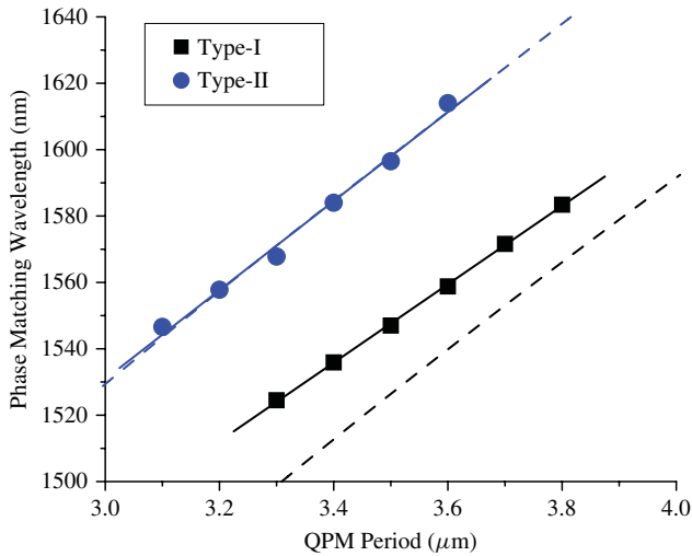
Fig. 4. Phase matching wavelengths for type-I and type-II SHG with several different QPM periods. Solid lines show the best linear fit to the measured data points. Dashed lines show the predicted phase matching wavelengths from the refractive index measurements in [16].
