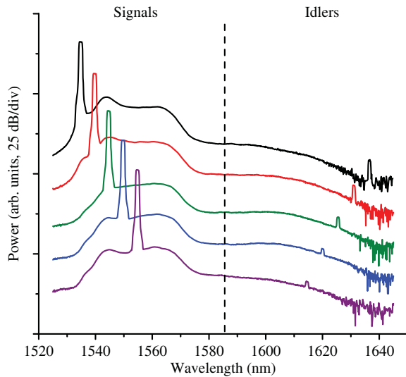
Fig. 6. Output spectra for type-I phase matching in a QPM waveguide for several signal wavelengths. The QPM period was 3.8 \mu\text{m} . The pump wavelength was initially set to 791.7 nm and adjusted by no more than \sim 0.5 nm to maximize idler generation. Signal wavelengths are shown on the left and the generated idler wavelengths are shown on the right.
