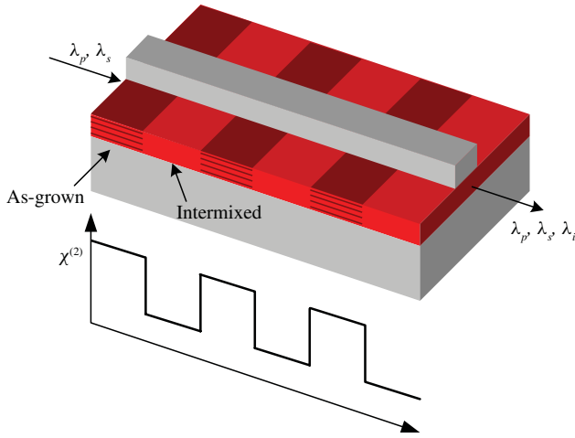
Fig. 1. Schematic of a domain-disordered quasi-phase matching waveguide. The superlattice core layer is patterned by quantum-well intermixing such that a grating with high (as-grown) and low (intermixed) \chi^{(2)} is formed to mediate the difference frequency generation process such that the idler wavelength ( \lambda_i ) is efficiently generated by the pump ( \lambda_p ) and signal ( \lambda_s ) wavelengths.
