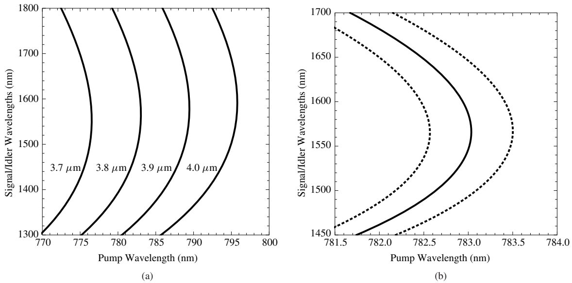
Fig. 2. Calculated tuning curves for a three-wave interaction in a type-I configuration (a) for the QPM grating periods \Lambda = 3.7\text{--}4.0\ \mu\text{m} (b) detail around the degeneracy point for \Lambda = 3.8\ \mu\text{m} . The short-dashed lines in (b) show the completely out-of-phase wavelength combinations for a 1 mm waveguide length.
